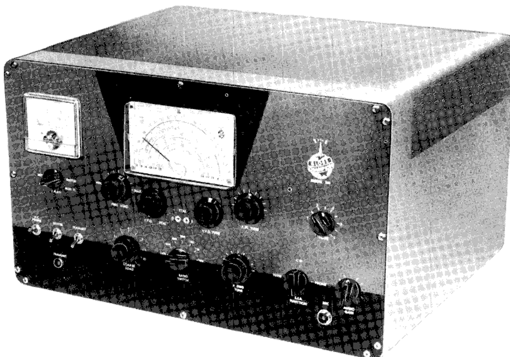
Globe Champion Transmitter Model 300
